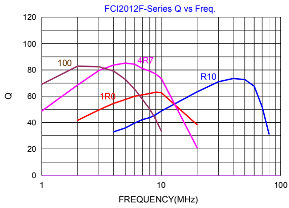
■ Q-Frequency Characteristics
