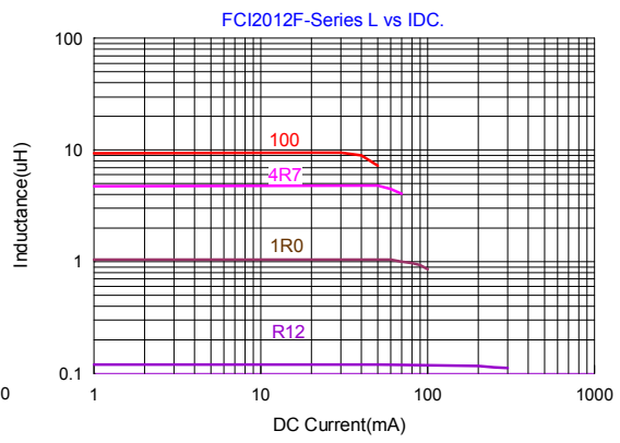
■ Inductance-Current Characteristics
